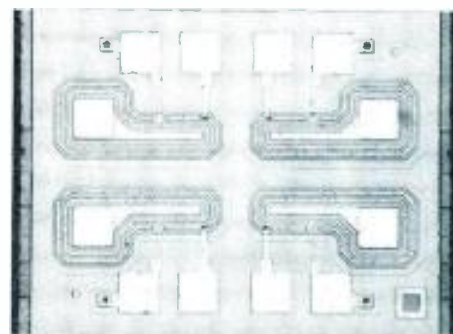
A magnified view of the circuit pattern for the SD5002 quad analog switch chip.
