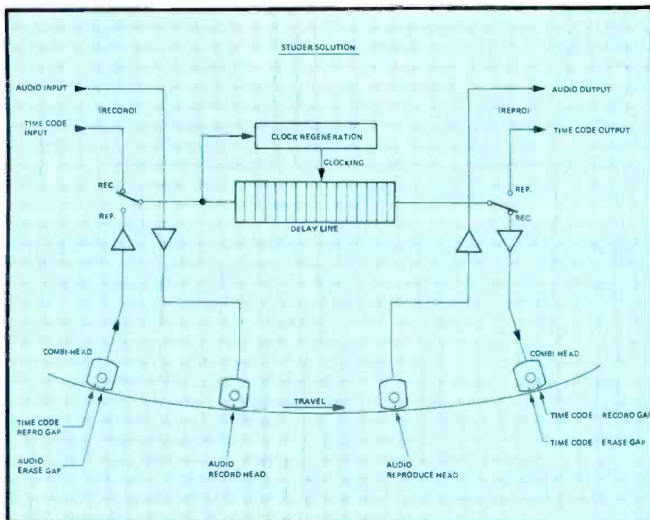
Figure 1. The Studer time coincident center channel SMPTE code system used in the A-810 tape recorder. According to the company, this arrangement keeps code-channel-to-audio-channel cross-talk at less than 90dB.
