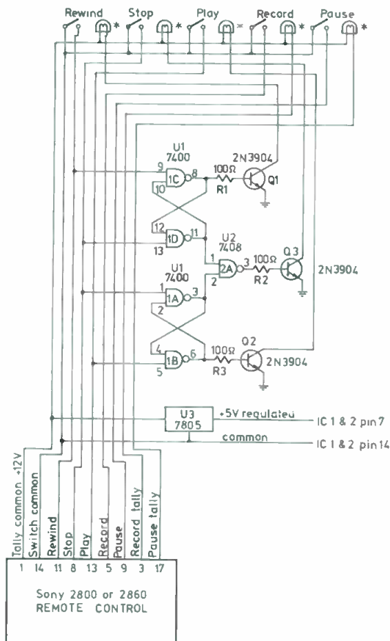
Figure 2. Remote control and tally for Sony 2800/2850.
